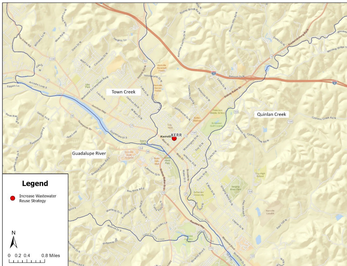
Figure 5C-3. J-29 City of Kerrville – Increase Wastewater Reuse Project Map
